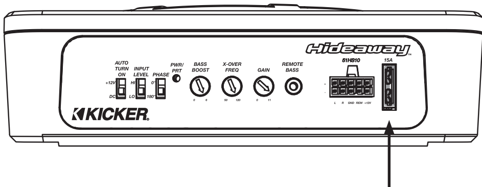
Fuse 15 Amperes
